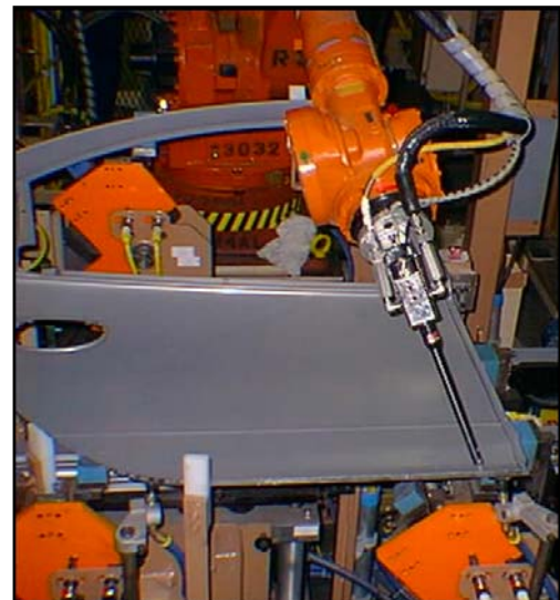
Automated Dispense Valve dispensing 2-Part adhesives and sealants
